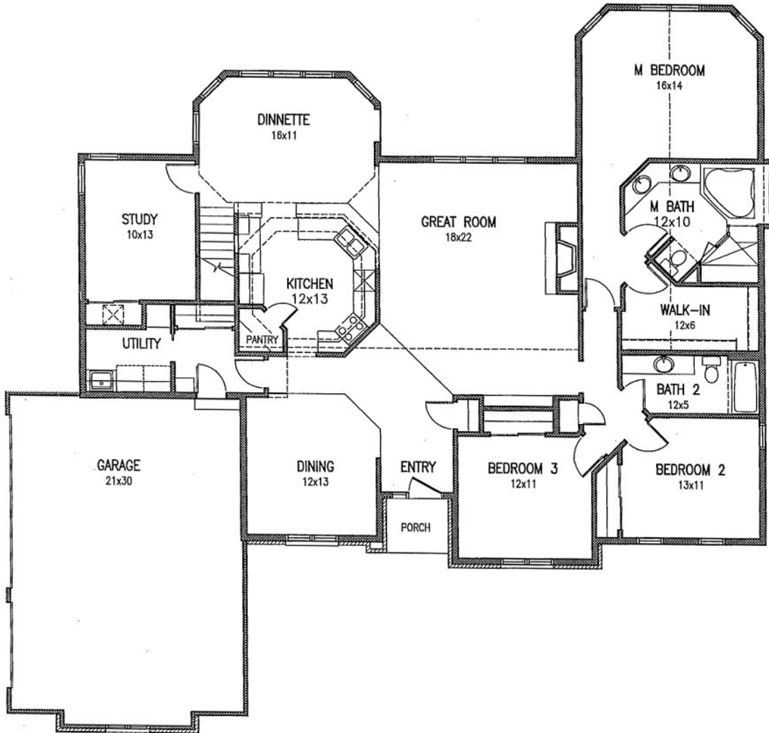
FIRST FLOOR PLAN 2,342 Sq Ft
