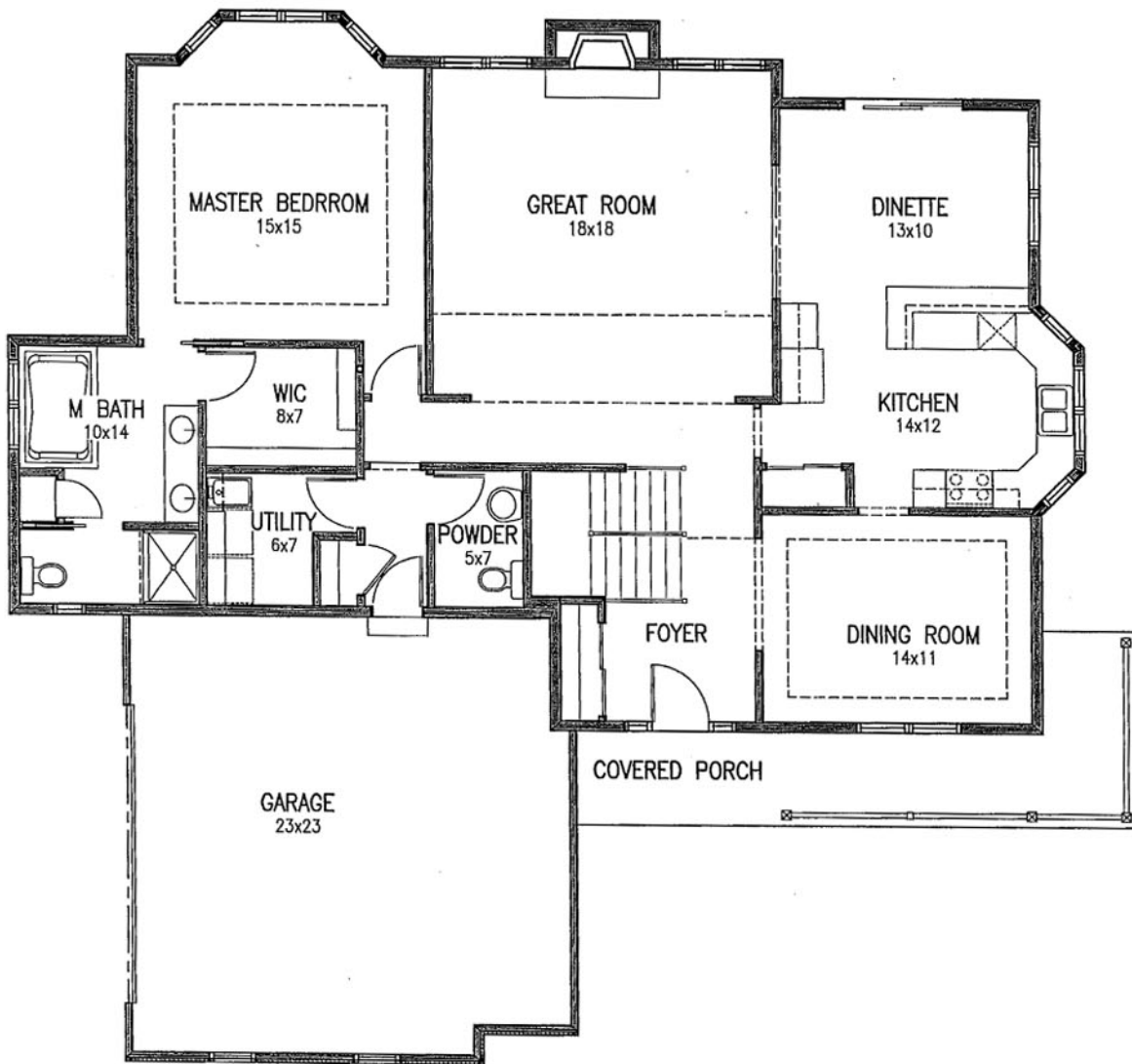
FIRST FLOOR PLAN 1,728 Sq Ft
